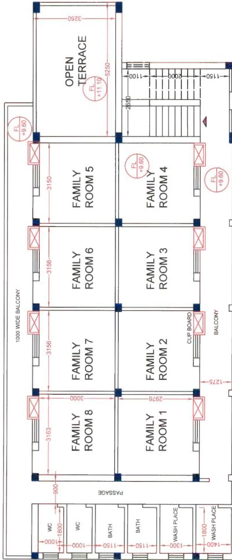
THIRD FLOOR PLAN FOR FOUR STORIED NIGHT SHELTER FOR 50 PERSON
