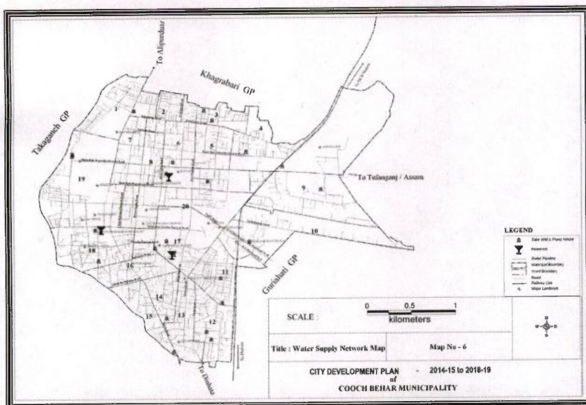
Water Supply Network Map
