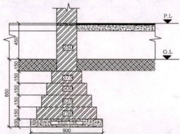
250 MM THK. BRICK WALL
