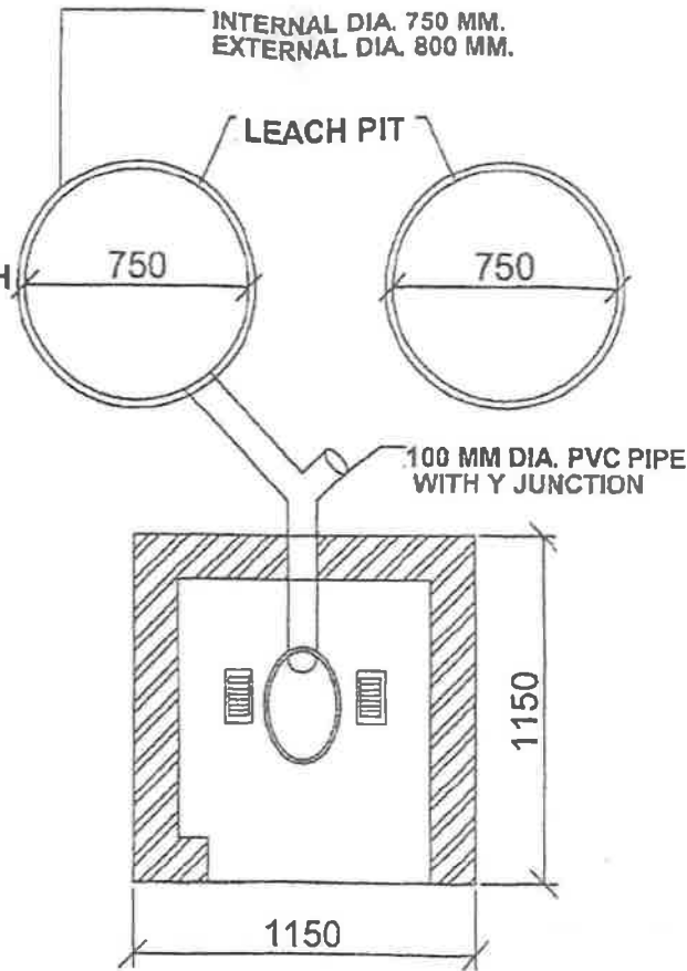
PLAN
