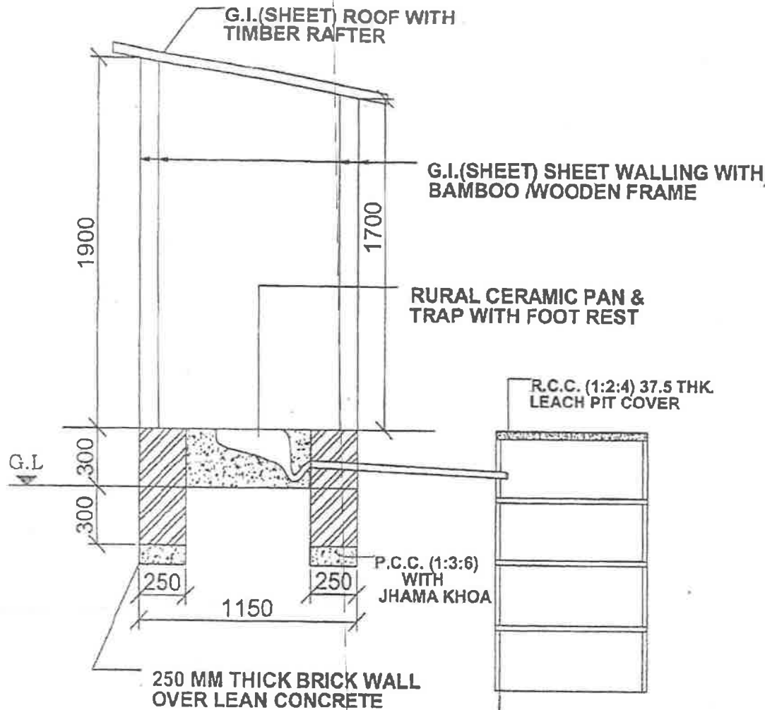
SEC. ELEVATION
