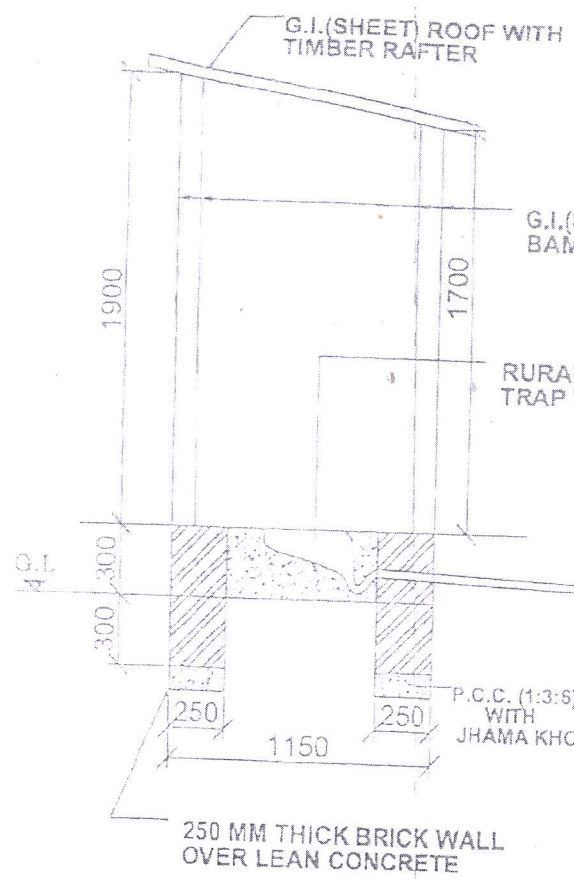
SEC. ELEVATION
