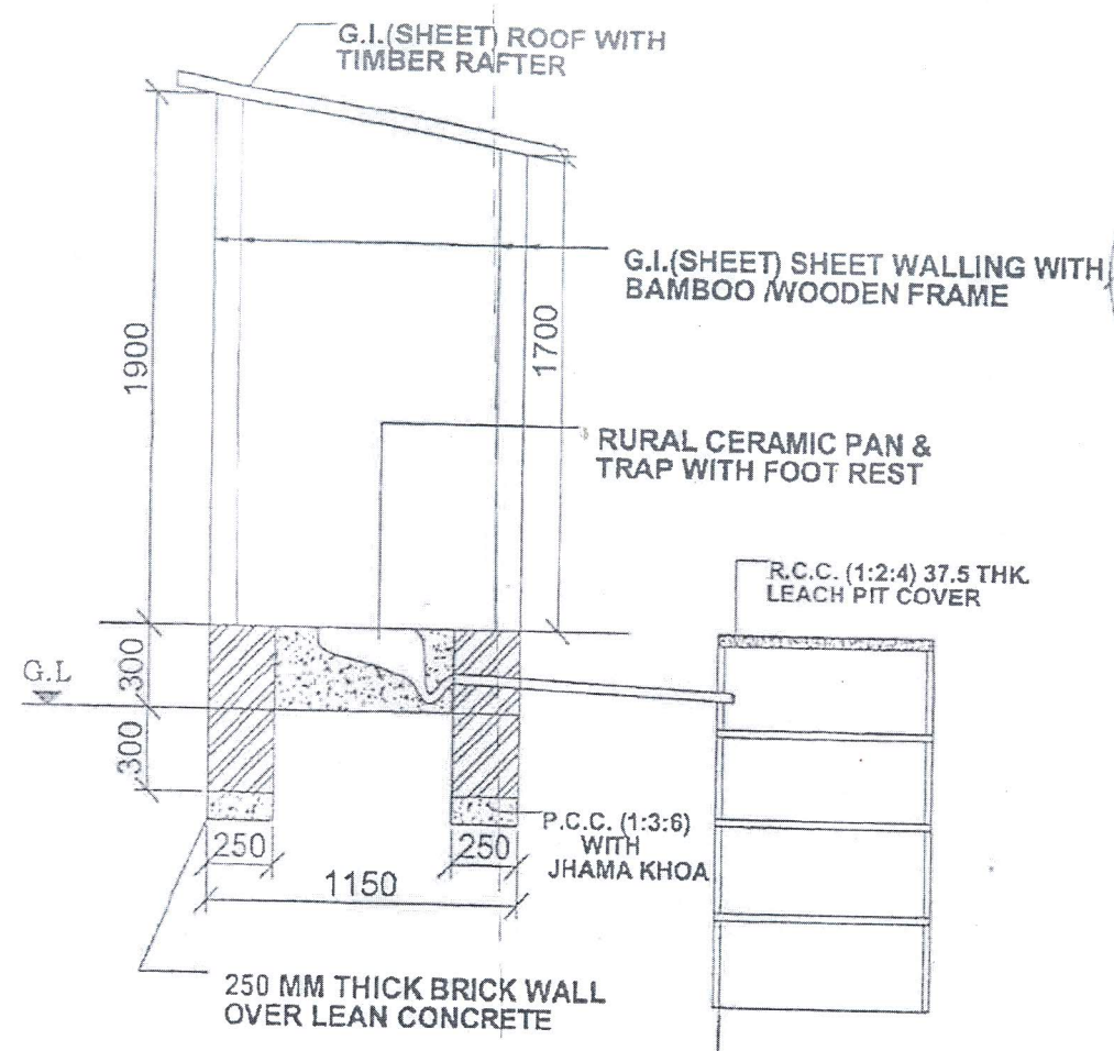
SEC. ELEVATION
