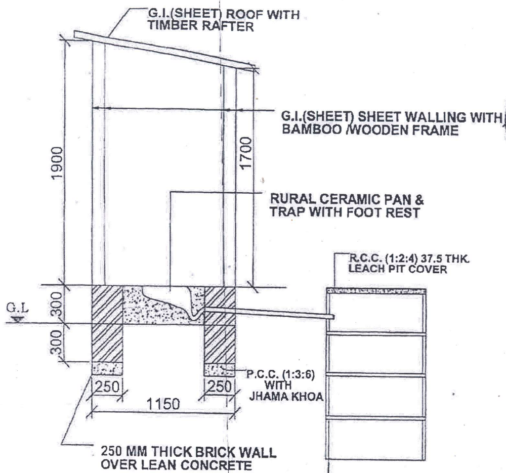
SEC. ELEVATION
